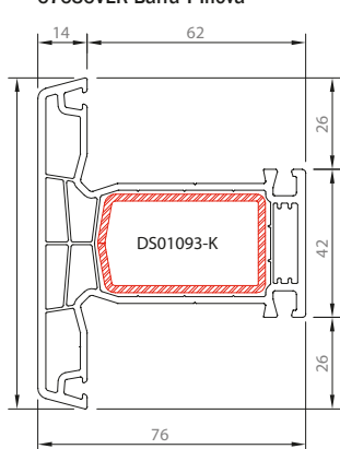
67636VER Barra T Inova
