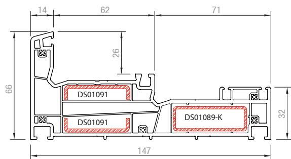
Marco Inova 61471VER
